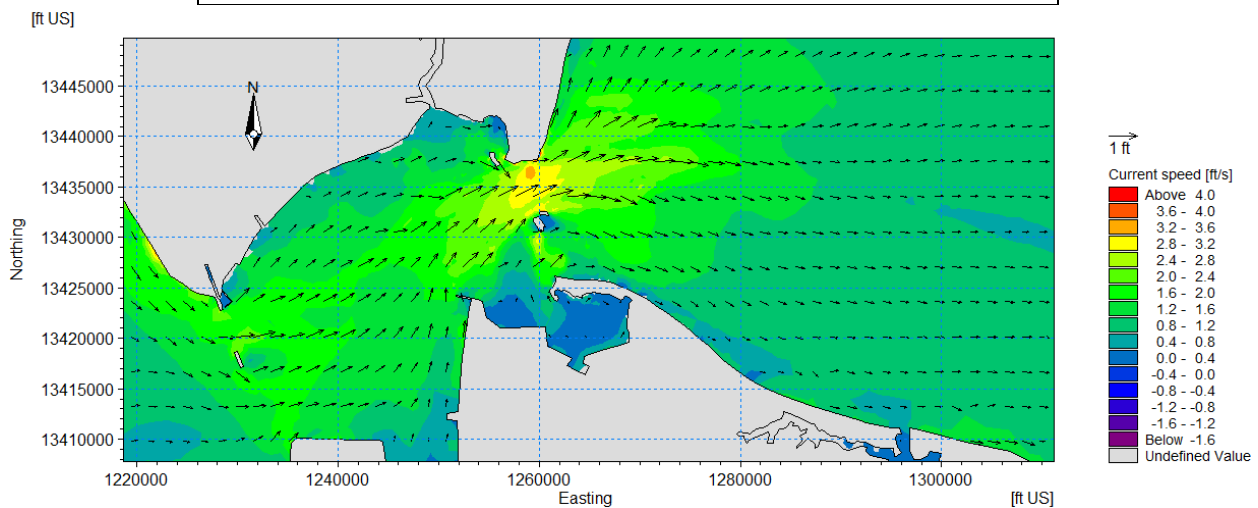
Figure 16.5.7-1 Hydrodynamic Model Operational Ebb Current Speed Plot
