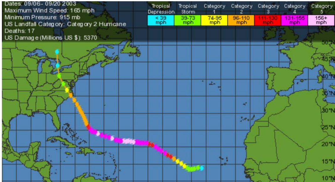
Figure 16.5.3-2 Track of Hurricane Isabel 2003 (From Weather Underground)
