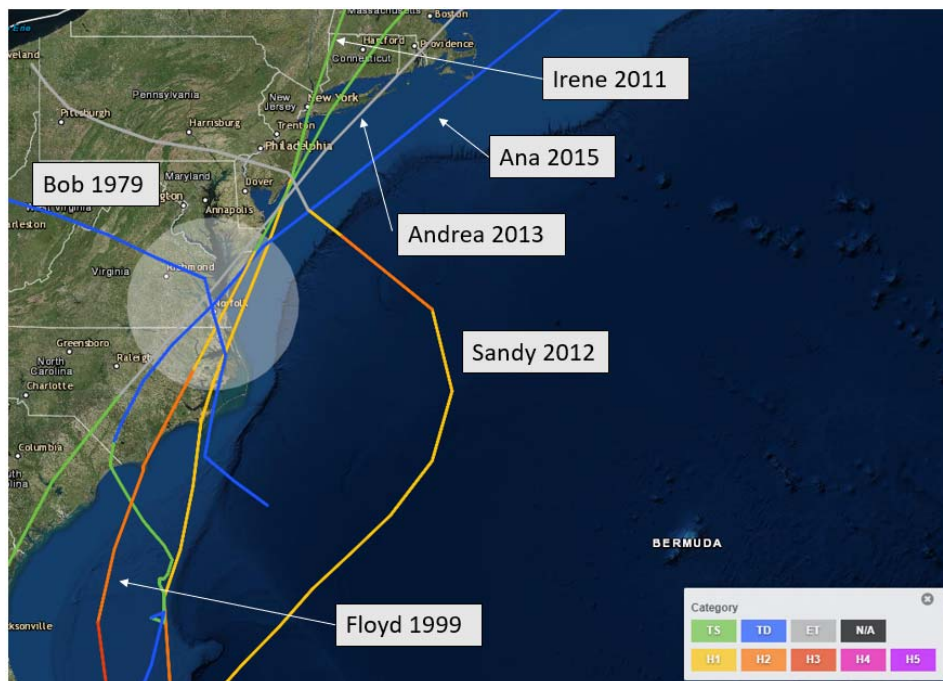
Figure 16.5.3-1 Tracks of 6 Hurricanes in the vicinity of the project site Over the Past 40 Years (NOAA)
