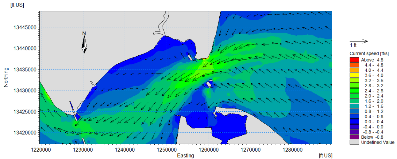
Figure 16.5.7-2 Hydrodynamic Model Operational Flood Current Speed Plot
